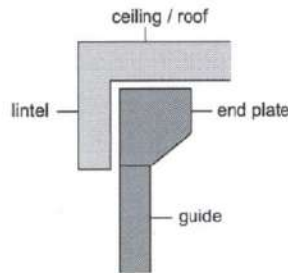
Face Fix
